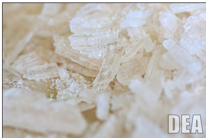
Figure 27. Crystal Methamphetamine
